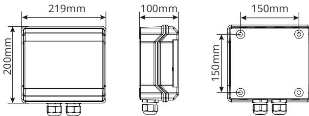
RCD for GW11K-HCA & GW22K-HCA
